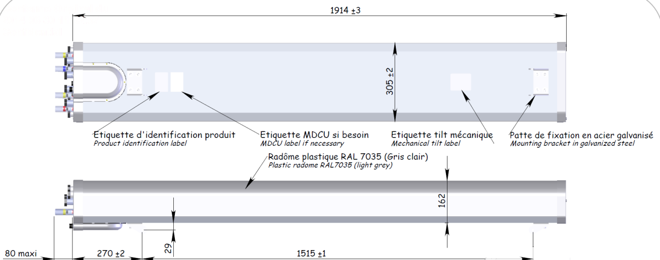
Location of the MDCU for RET control
