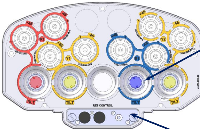
Location of the MDCU for RET control
